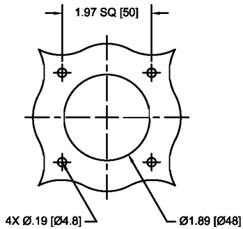
Mounting Dimensions for 2.84" x 2.84" plastic mounting bezel
