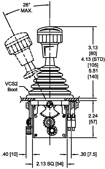
CS1 with internal potentiometer and (2) 5A SPDT Micro Switches each axis
