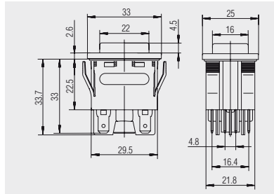
Quick-connect terminal 4.8 1673.5501
