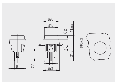
Quick-connect terminal 2.8 5000.0101, 5000.0103 and 5000.0104
